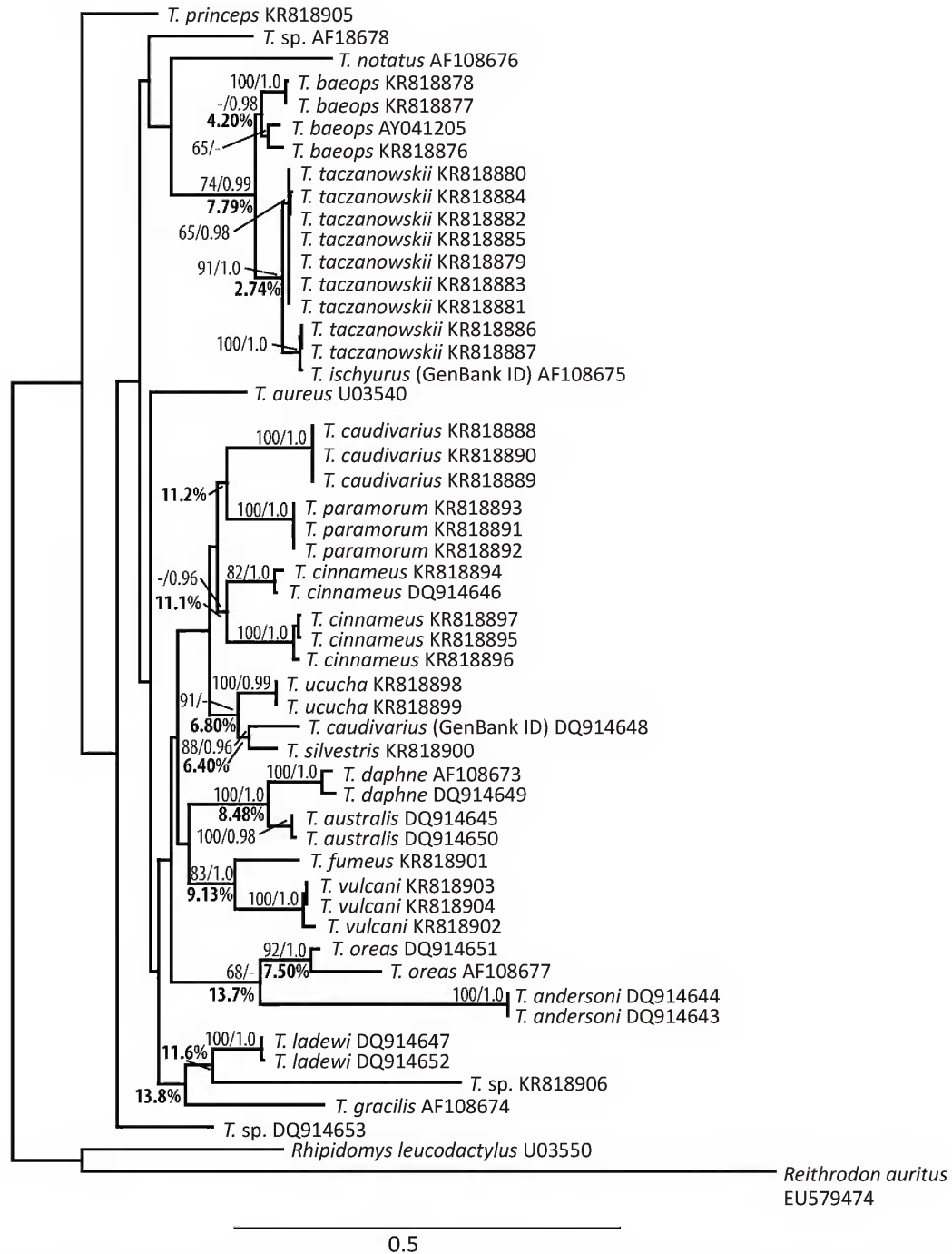
Figure 2. Maximum likelihood tree from analysis of Cytb sequences, the scale bar represents nucleotide substitutions per site. Numbers at branch tips are GenBank accession numbers; numbers above branches are maximum likelihood bootstrap proportions/Bayesian inference posterior probabilities, respectively. Bootstrap proportions less than 50% and posterior probabilities less than 0.95 are not shown or are designated by a dash. Bold numbers below selected branches are average Kimura 2-parameter genetic distances between the two sister clades subtended by the branch. If GenBank accessions from previous studies designate a taxon name that conflicts with taxonomy in this study, “(GenBank ID)” is included following the taxon name.
